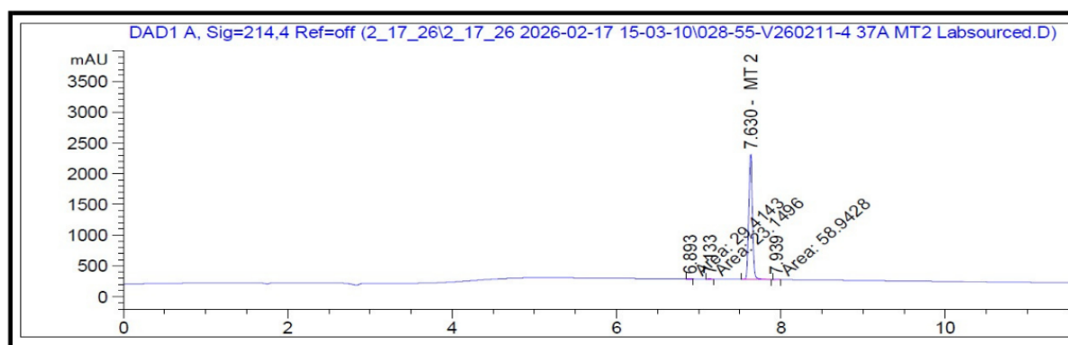
Chromatogram for Vial "A" shown above.
